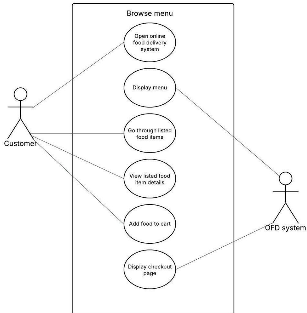
Browse menu use case diagram
